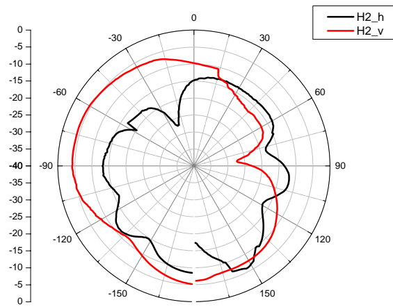
H (XZ) plane radiation pattern
