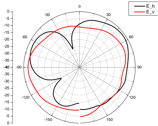
E (YZ) plane radiation pattern
